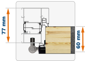
ALUTHERM 60 aluminium frame
