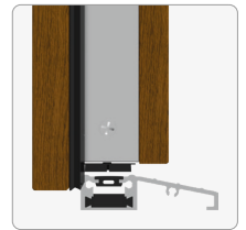
4 sides rebated Low, aluminium threshold with thermal break
