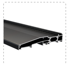
Cill, 4 sizes available: 120 mm, 150 mm, 180 mm, 230 mm
