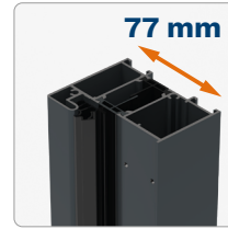
ALUTHERM 75 aluminium frame
