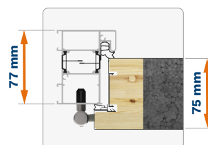
ALUTHERM 75 aluminium frame
